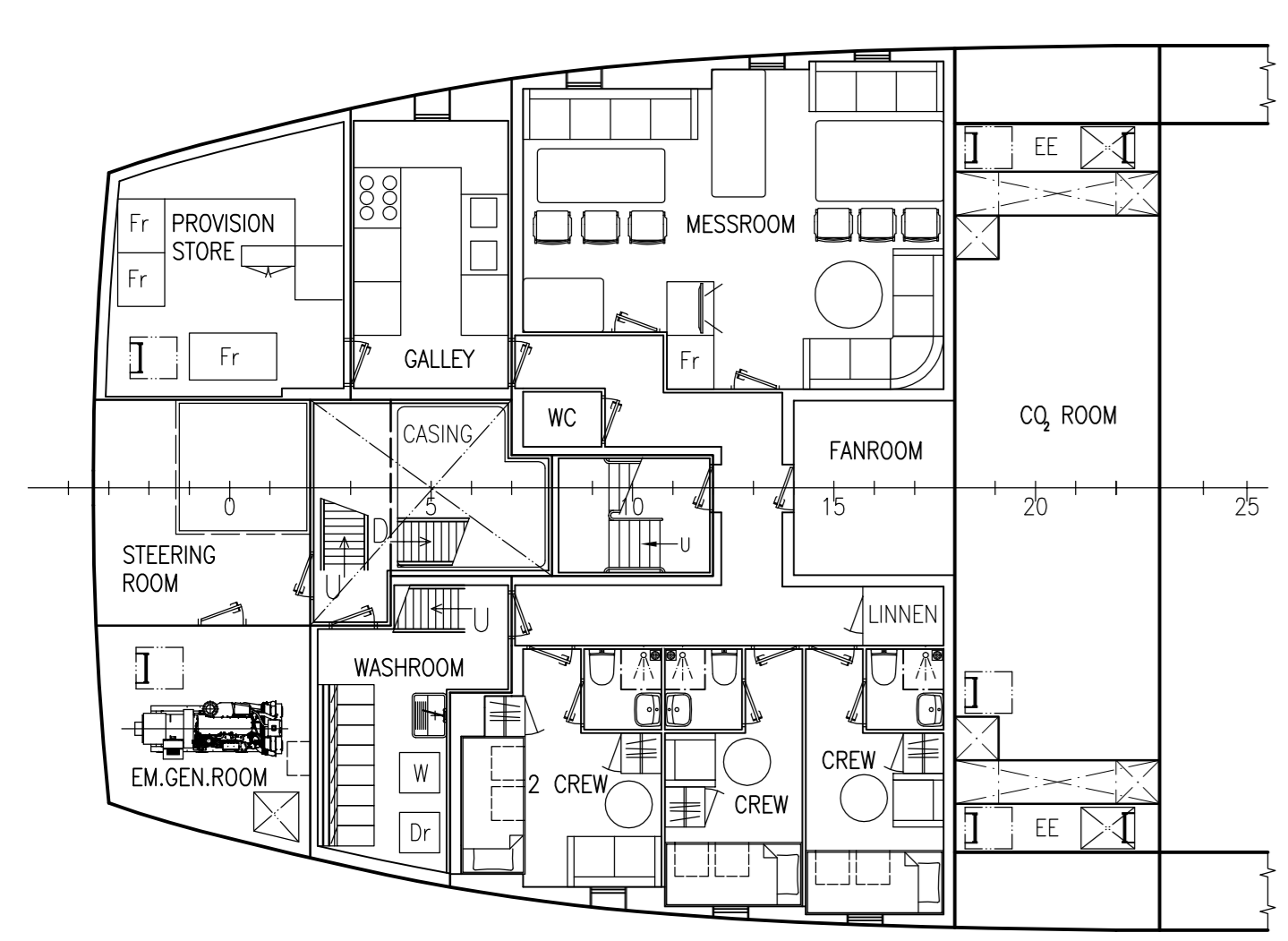
ACCOMMODATION DECK
