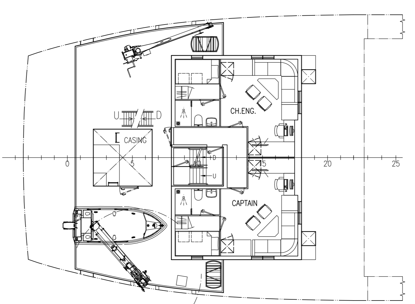
BOAT DECK
