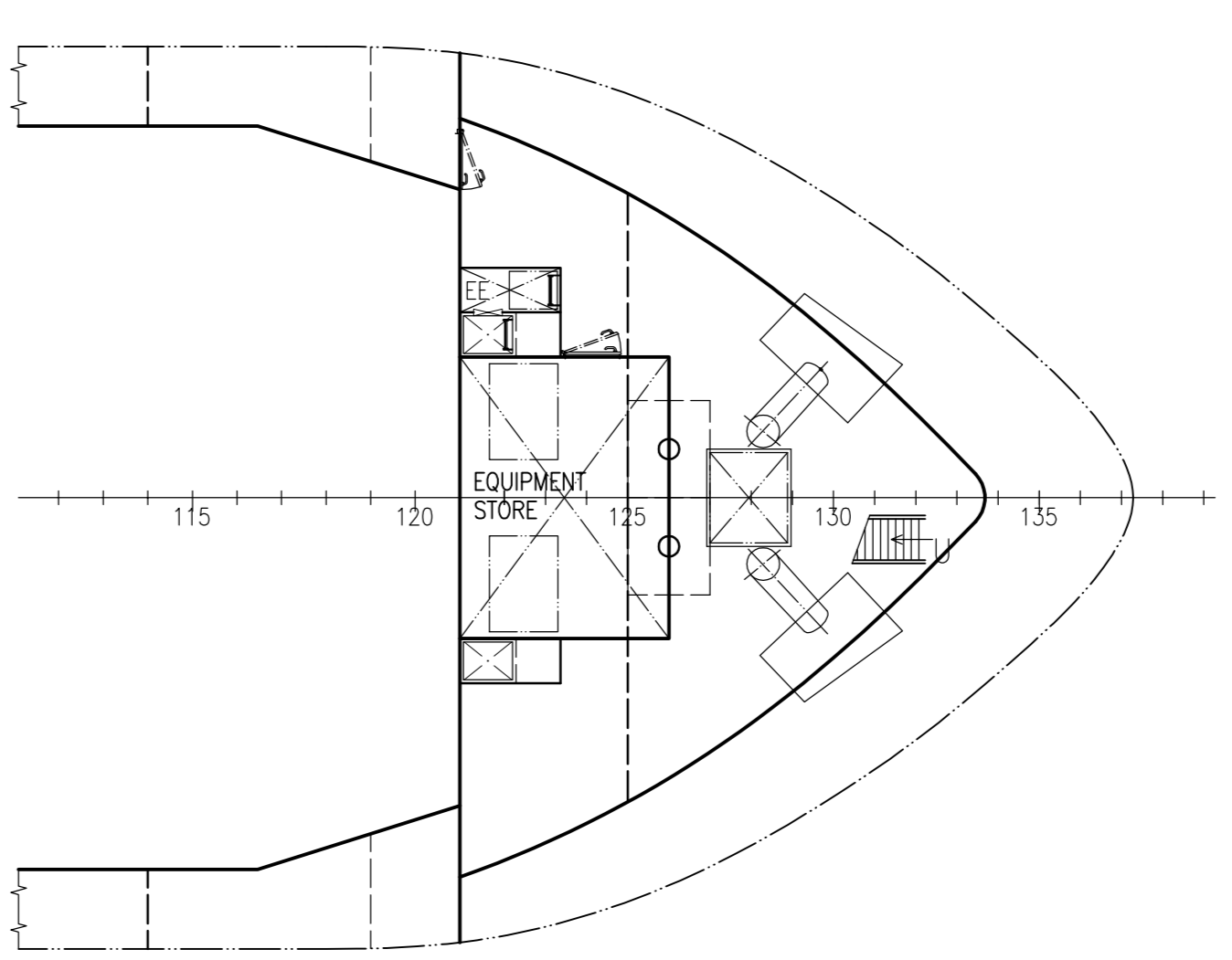
MAIN DECK
