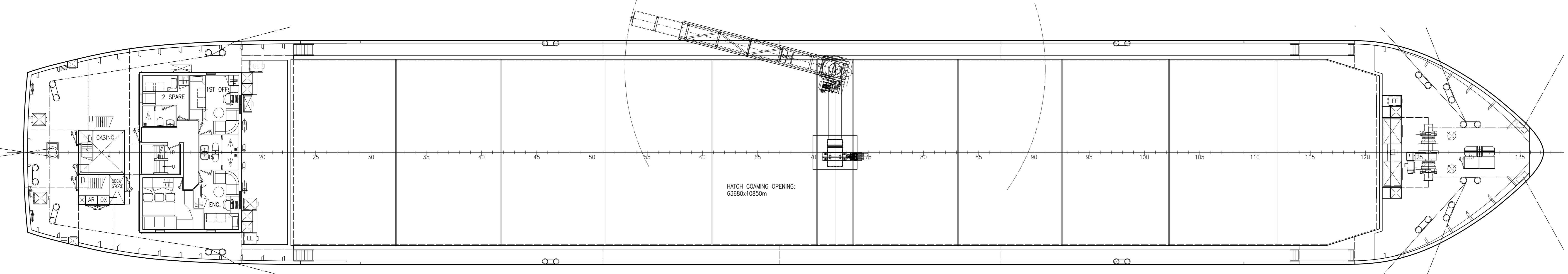
POOP DECK
